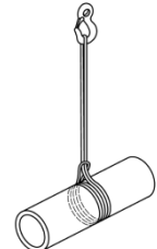
Figure C.1 – Elingage baguet double
