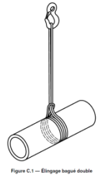
Figure C.1 - Elingage bagué double
