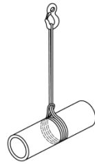
Figure C.1 – Elingage baguet double
