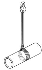
Figure C.1 – Elingage haquet double
