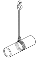
Figure C.1 – Elingage linga double
