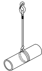
Figure D.2 — Élingue baquet double
