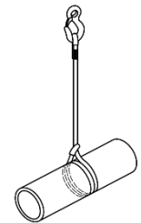
Figure D.2 — Elingage baquet double
