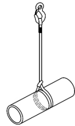
Figure D.2 — Élévation baguet double
