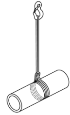
Figure C.1 – Elingage haquet double
