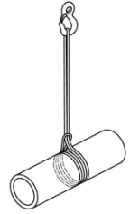
Figure C.1 – Élingage bouge double
