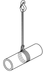
Figure C.1 — Élingage bague double
