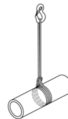
Figure C.1 – Elingage bandes double
