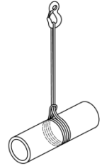
Figure C.1 – Elingge baguet double
