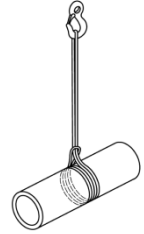
Figure C.1 – Elingsge ligout double
