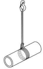
Figure C.1 — Élingage bague double
