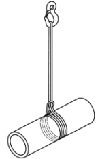
Figure C.1 — Elingage biquet double
