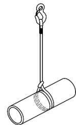
Figure D.2 — Étringale baquet double
