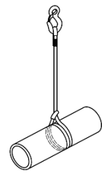
Figure D.2 — Élingage bagou double
