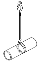
Figure D.2 – Élingage bagout double
