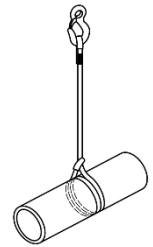
Figure D.2 — Élingage baguê double
