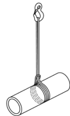
Figura C.1 – Elingage lingué double
