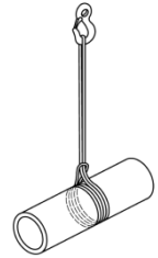
Figure C.1 — Eslingage bougé double
