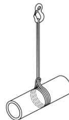
Figure C.1 – Elingage bague double
