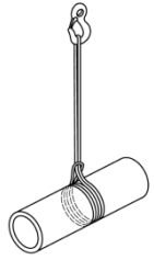
Figure C.1 – Étrappe bougé double
