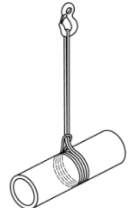
Figure C.1 — Lifting basket double
